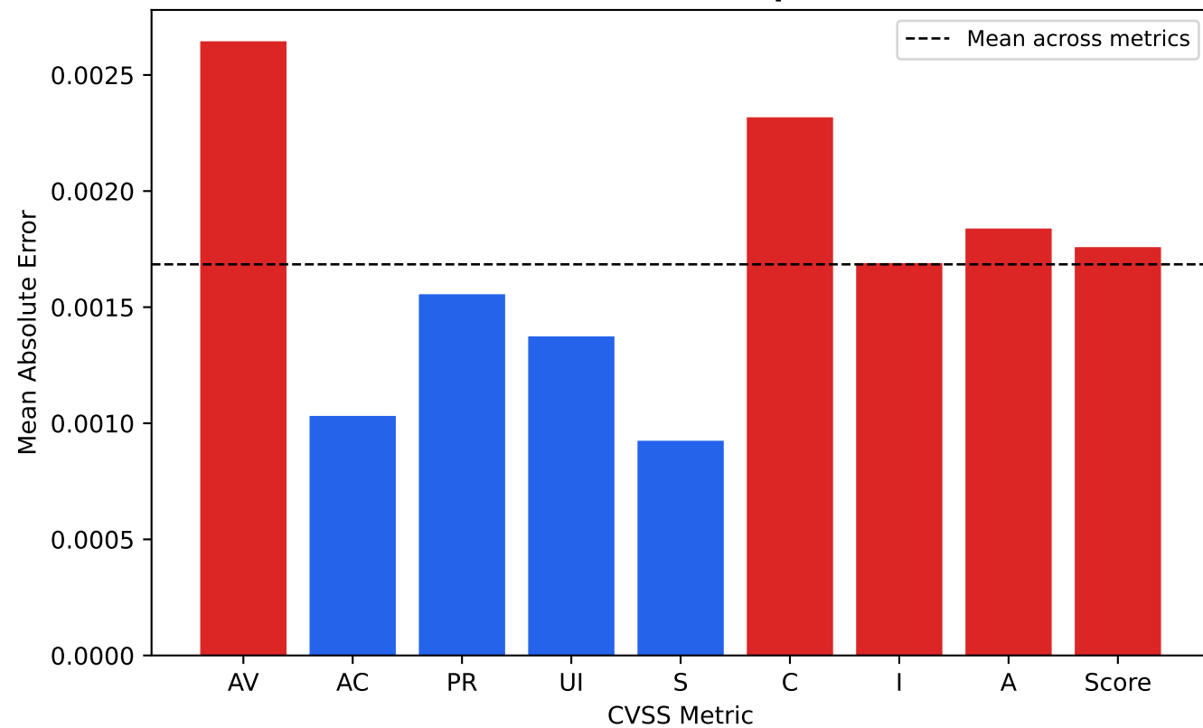
Mean Reconstruction Error per CVSS Metric
